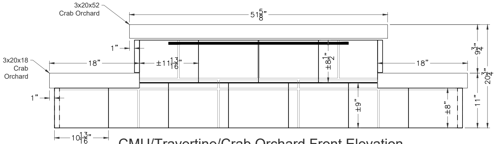
CMU/Travertine/Crab Orchard Front Elevation
