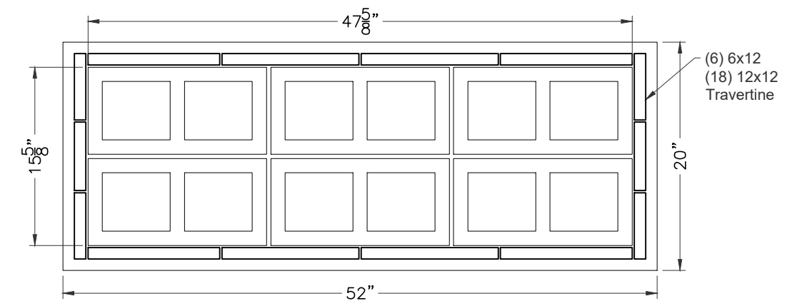
CMU/Travertine/Crab Orchard 2nd Row Plan View
