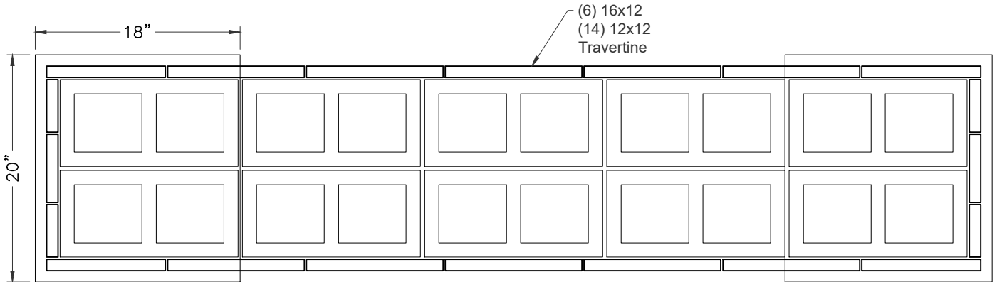
CMU/Travertine/Crab Orchard 1st Row Plan View
