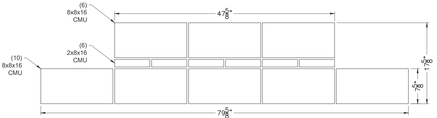
CMU Front Elevation
