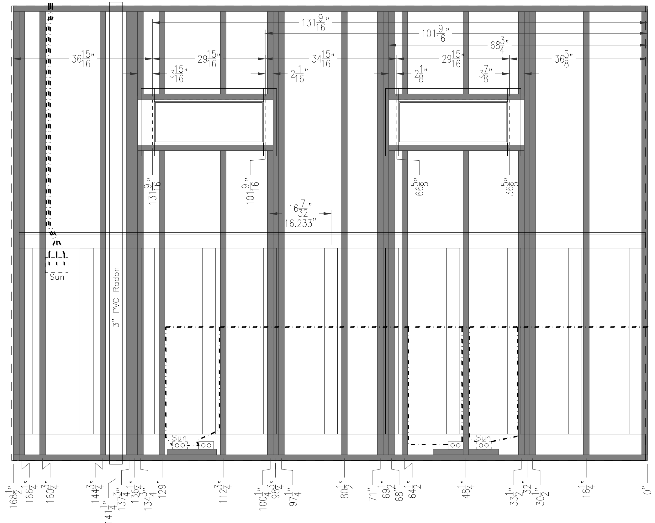
Dining Room - East Wall Stud & Wainscoting Location
