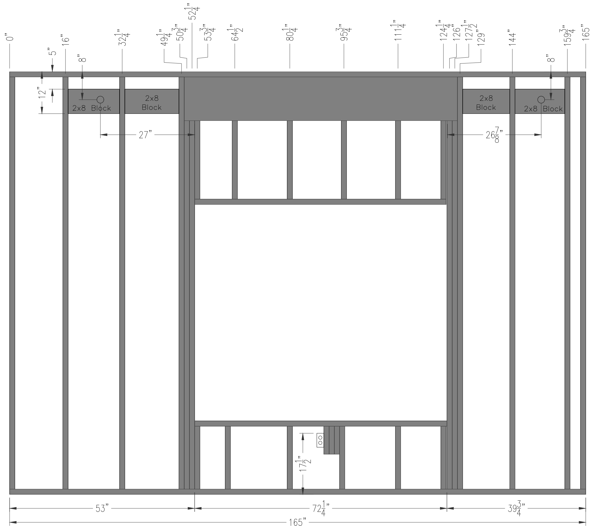
Living Room - West Wall Stud Location
