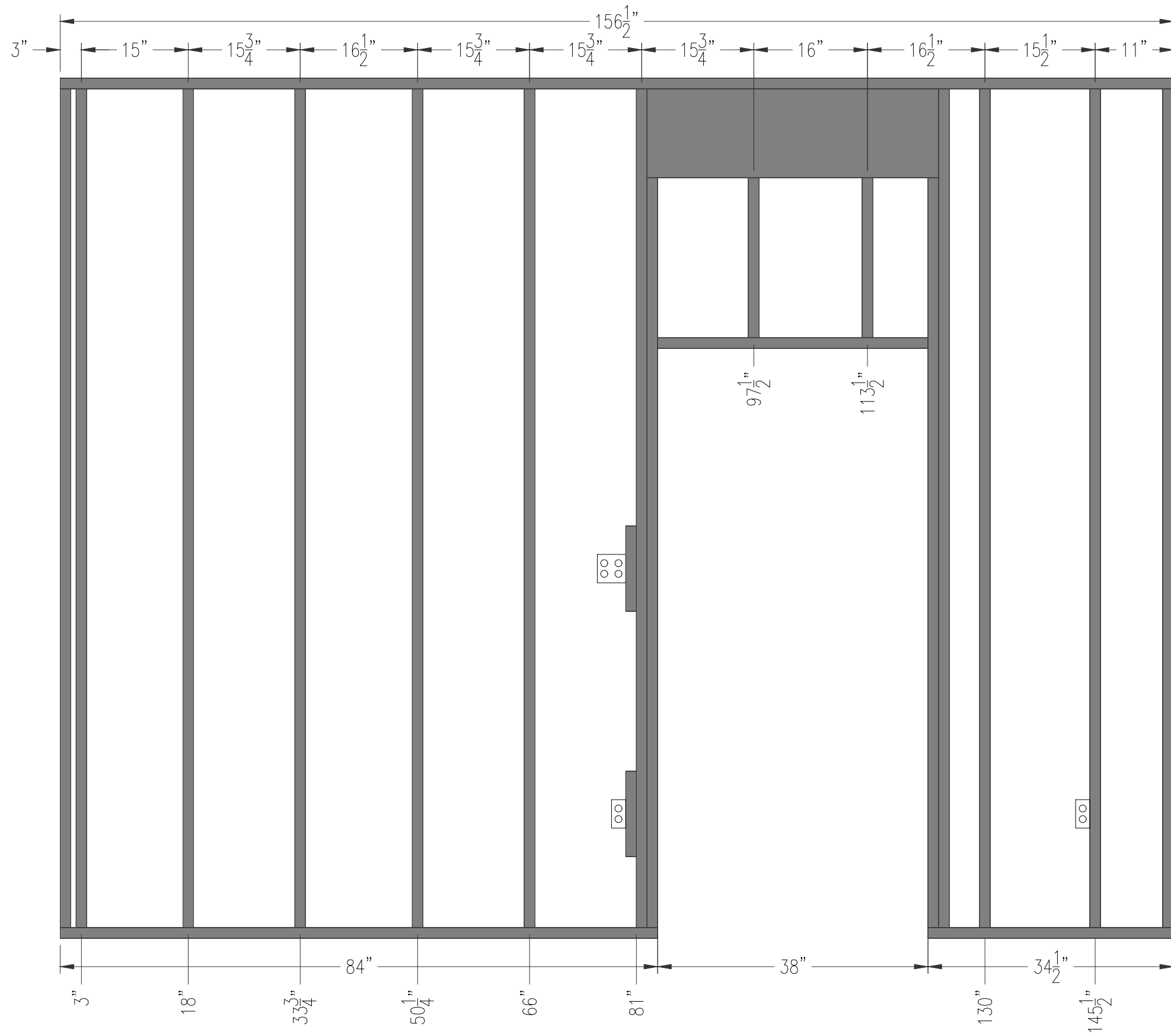
Master Bedroom - East Wall Stud Location
