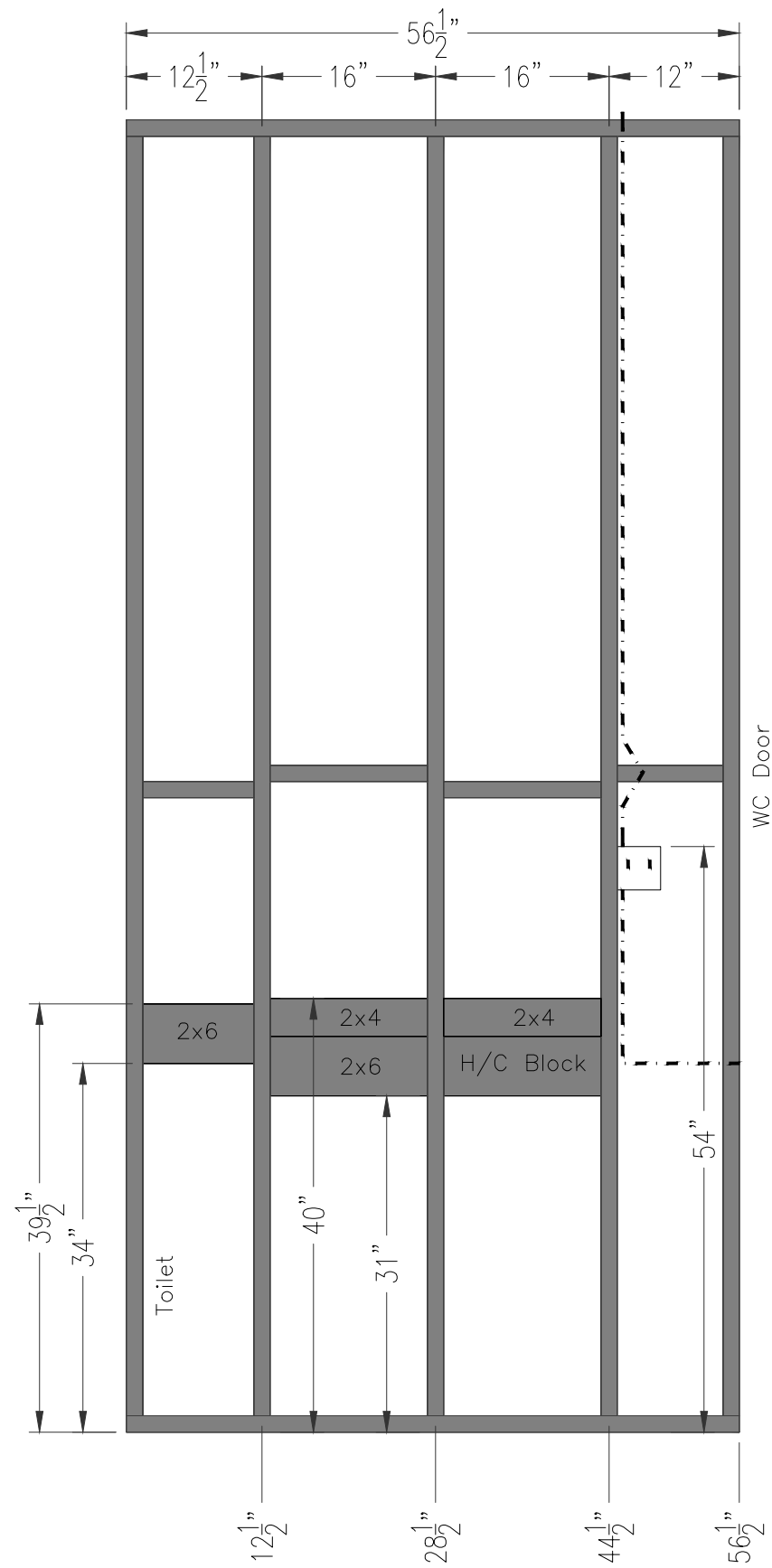
Master WC - East Wall Handicap Blocking
