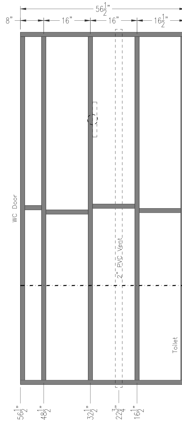
Master WC - West Wall Stud Location
