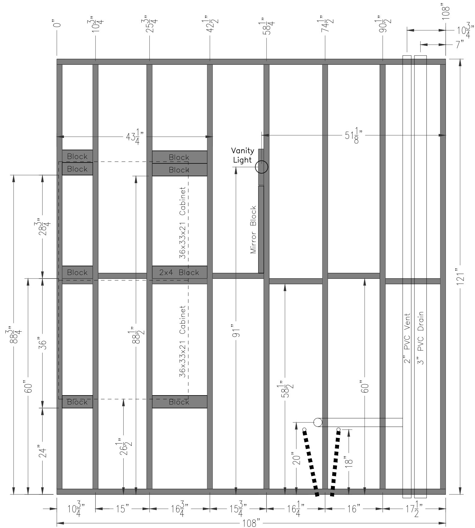
Pool Bath #3 - East Wall Floating Cabinet & Vanity Mirror Blocking
